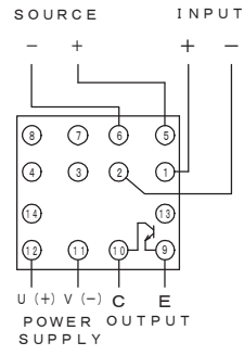
CONNECTION DIAGRAM
